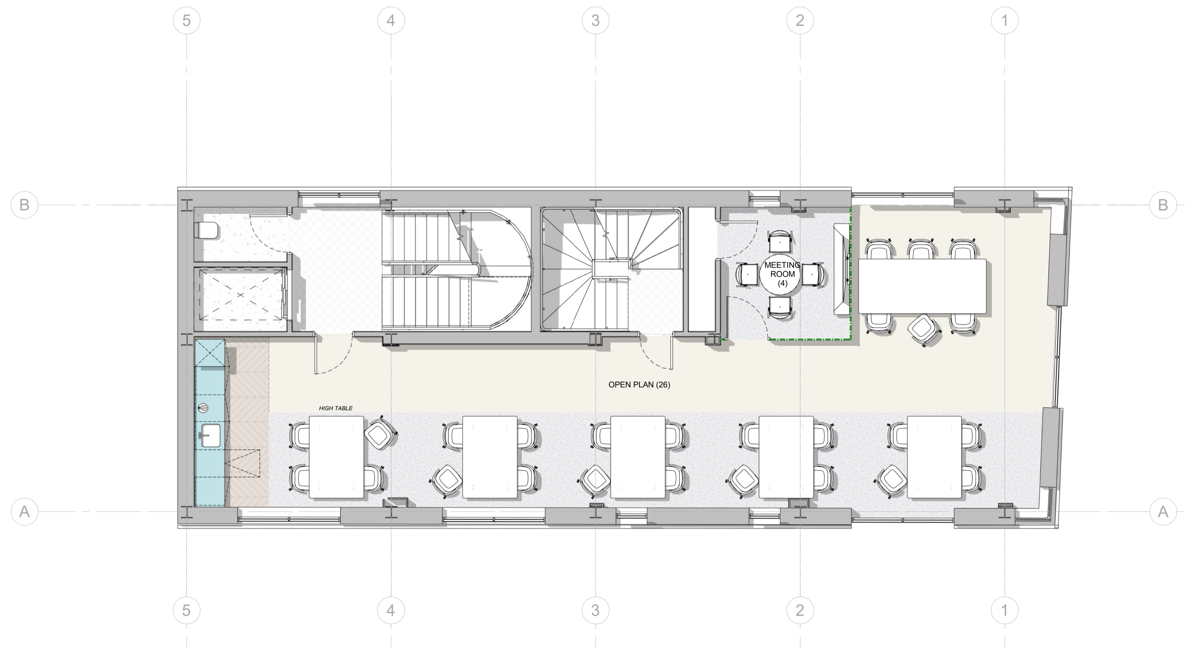
1 GENERAL ARRANGEMENT - LEVEL 01 1400 DESKS 1:50
