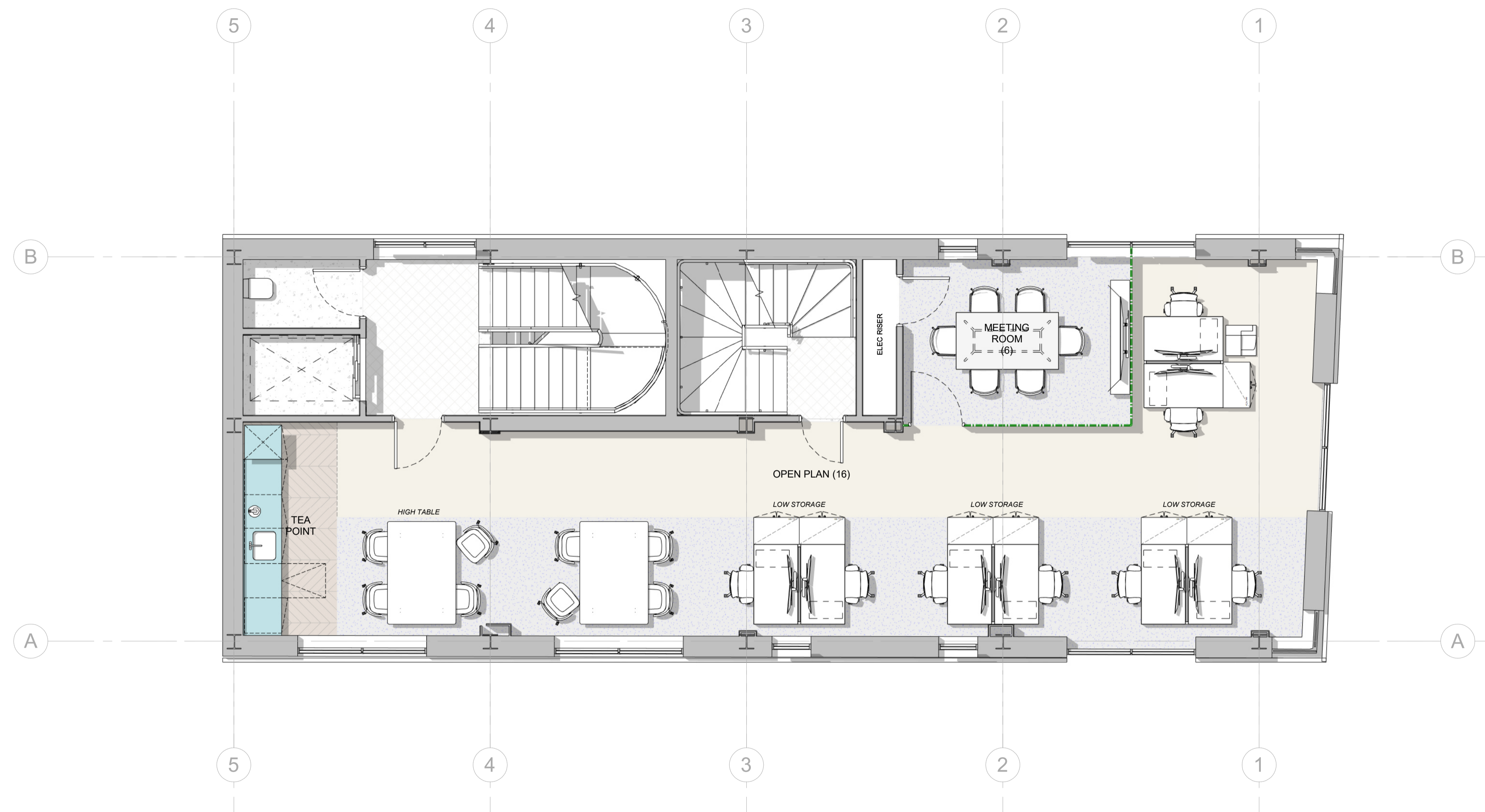
GENERAL ARRANGEMENT - LEVEL 01 1400 DESKS & TOUCHDOWN 1: 50
